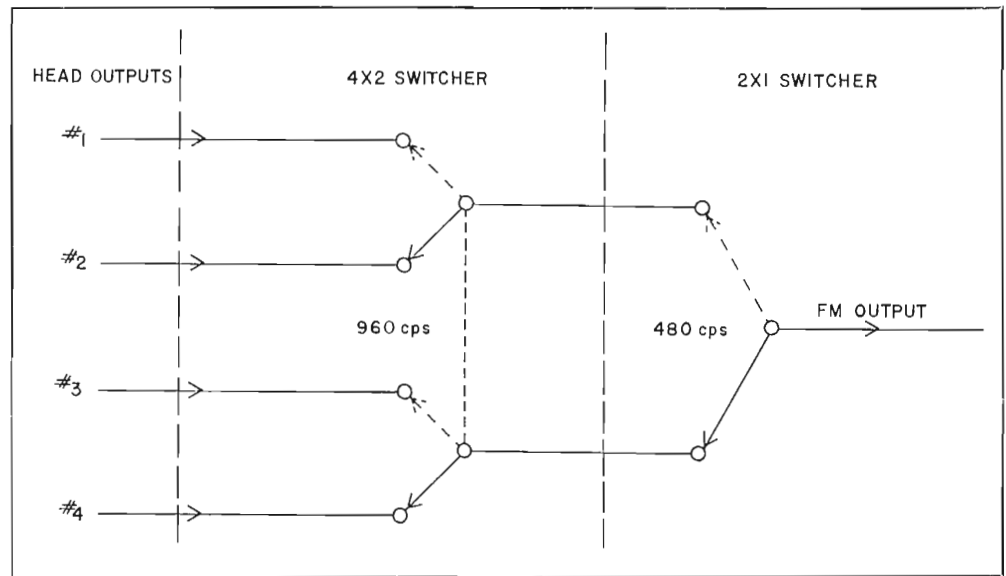
FIG. 4. Simplified schematic of FM switcher module.
