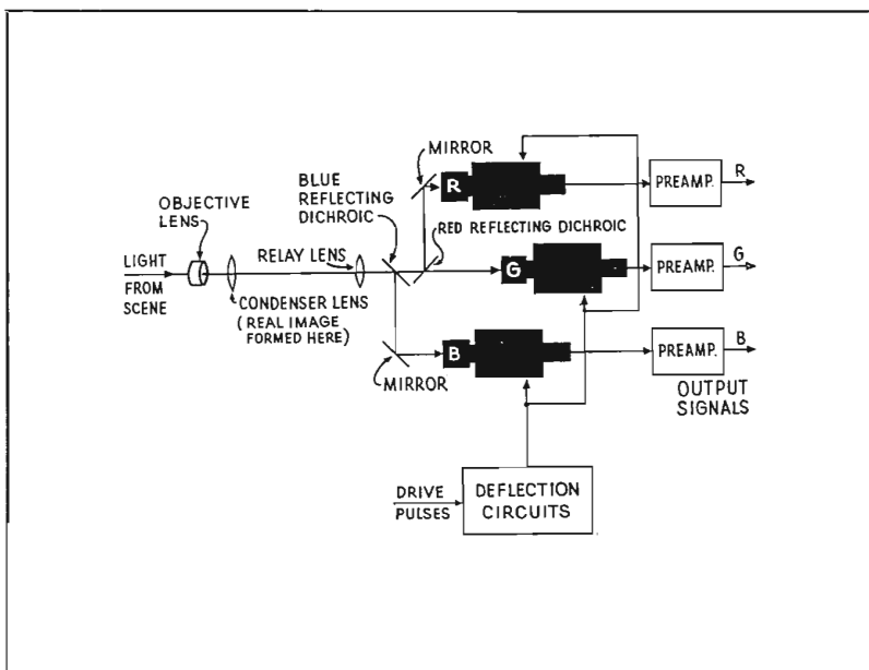
FIG. 2. Color camera components.
