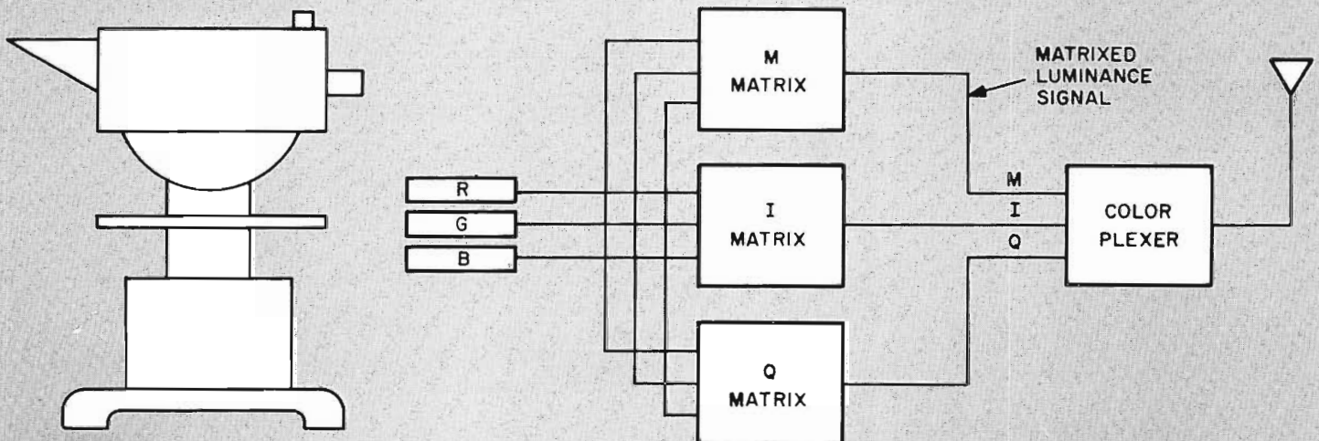
Block diagram showing how the luminance tube supplies monochrome signal simplifying the camera matrixing circuitry.
