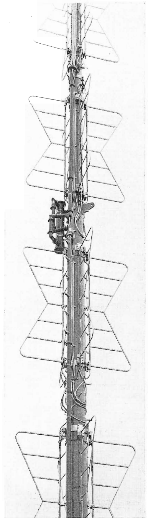
FIG. 8. View of antenna showing rigid 3/8-inch transmission lines feeding the combiner (center), and 7/8-inch Styroflex lines that feed batwing elements.
