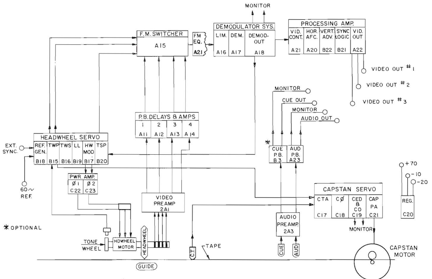
FIG. 2. TR-3 Functional Diagram.
