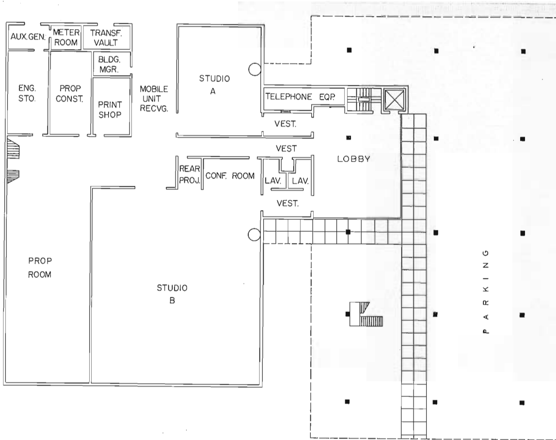
▲ FIG. 8. FIRST FLOOR PLAN.
