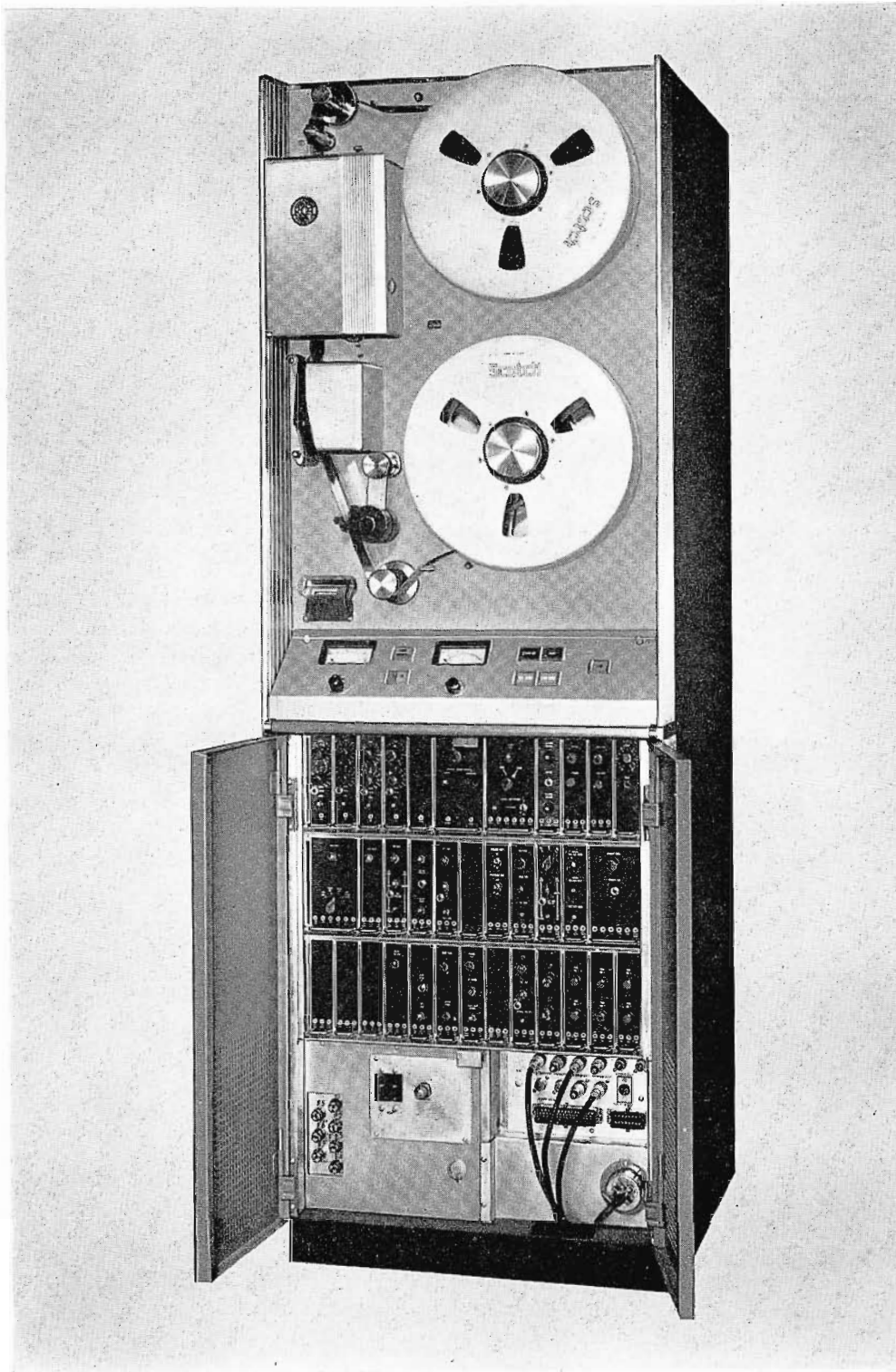
FIG. 1. TR-3 TV Tape Player.
