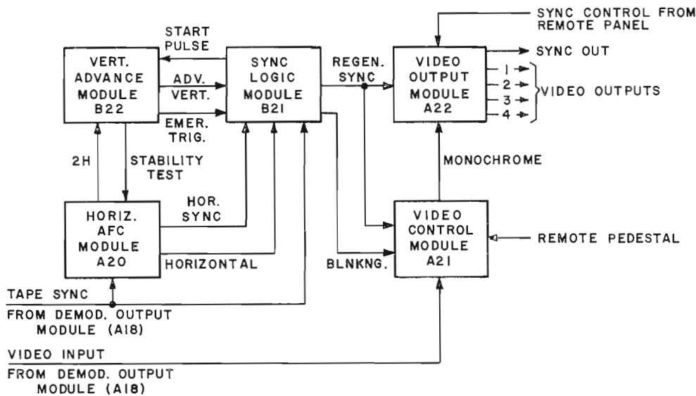
FIG. 6. Simplified block diagram of processing amplifier.
