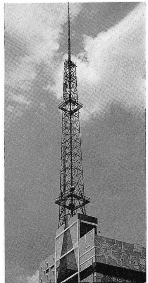
FIG. 9. Mexico City TV tower supports diplexed four-section Superturnstile for Channels 4 and 5.
