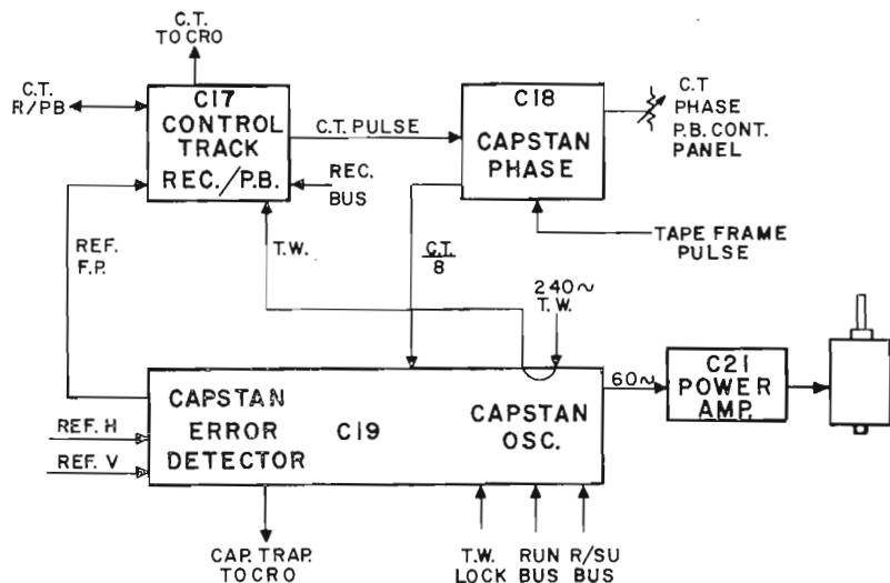
FIG. 8. Diagram of capstan servo.
