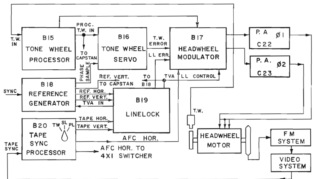
FIG. 7. Diagram of headwheel servo.
