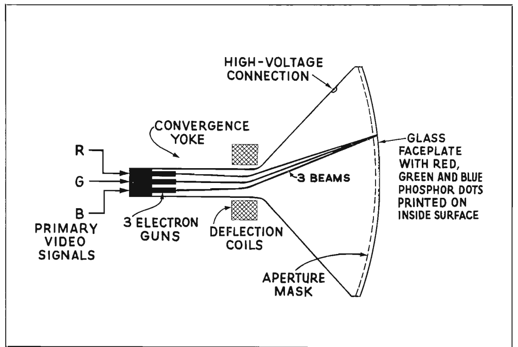
FIG. 5. Three-gun color kinescope.
