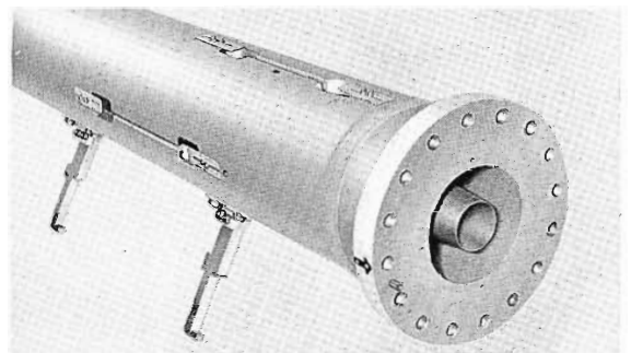
View showing simple design of "Pylon" Antennas
