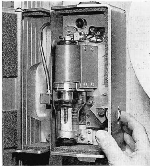
FIG. 12. Vacuum guide adjustment.
