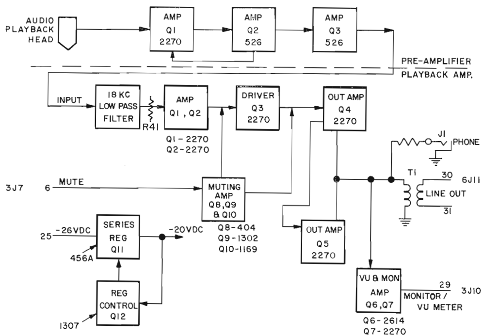
FIG. 10. Block diagram of TR-3 audio system.
